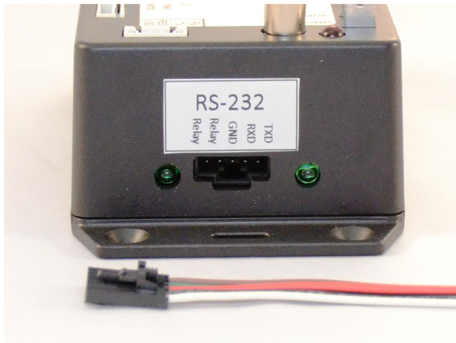
Picture 1: MODBUS Interface (default RS232)
